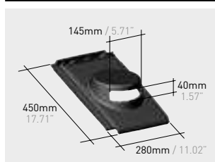
Q87*K | Planum chimney / Pipe tile klinker
