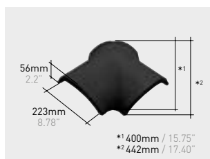
Q55*K | Round 3 way ridge female klinker
