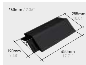
Q90*K | Atica ridge 120° klinker
