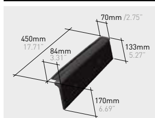
Q88*K | Planum right side course / Rake klinker
